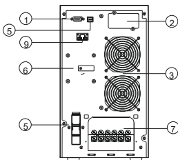
EOT-0010KVA-1-L
